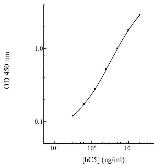
Human Complement C5 Standard Curve
